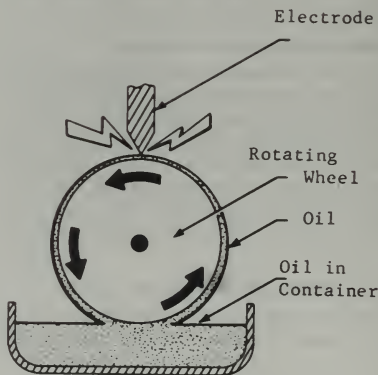
FIGURE 10-74. Oil Sample
